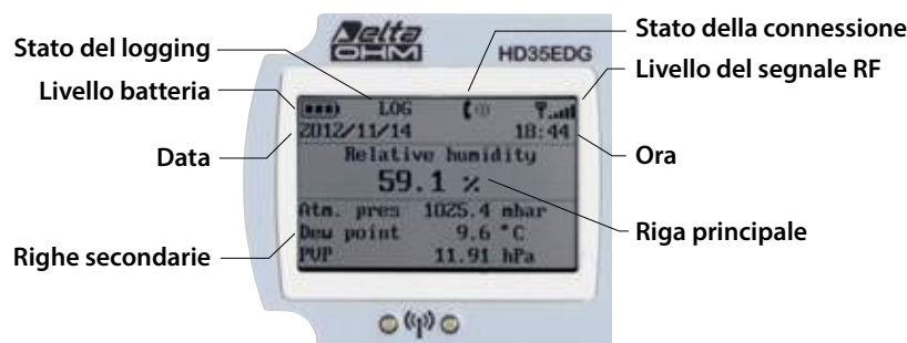
Graphic LCD
